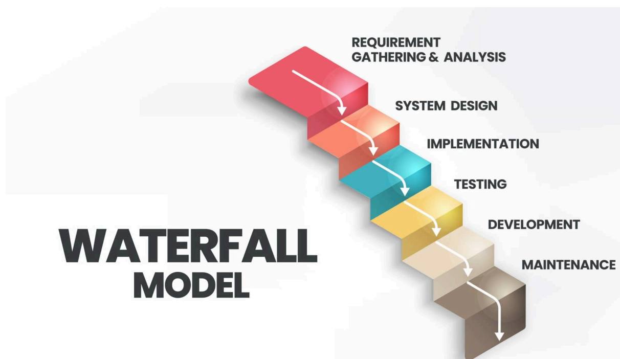
Figure 2.1 : Waterfall Model
